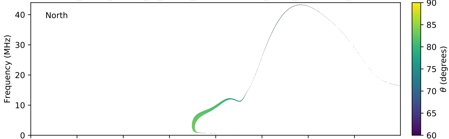
expres_earth_jupiter_io_jrm09_lossc-wid1deg_3kev_20100802_v01.cdf
