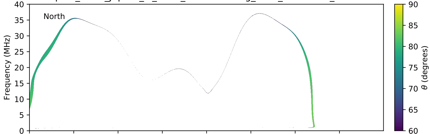
expres_earth_jupiter_io_isaac_lossc-wid1deg_3kev_20100829_v01.cdf
