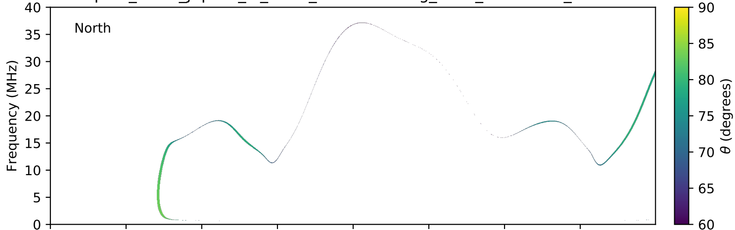
expres_earth_jupiter_io_isaac_lossc-wid1deg_3kev_20100827_v01.cdf
