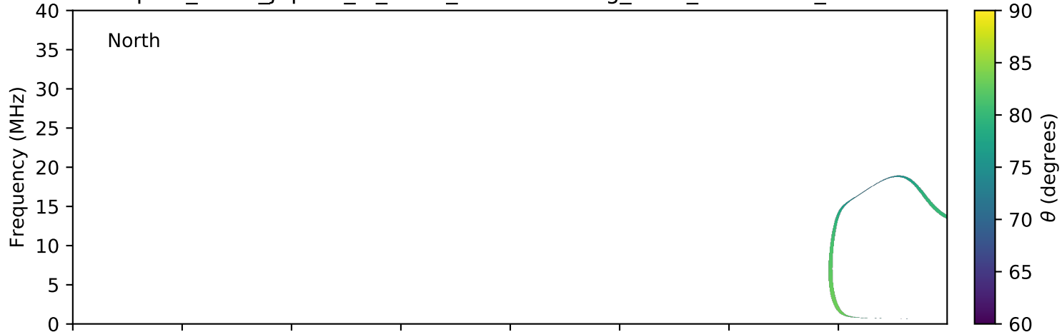
expres_earth_jupiter_io_isaac_lossc-wid1deg_3kev_20100821_v01.cdf
