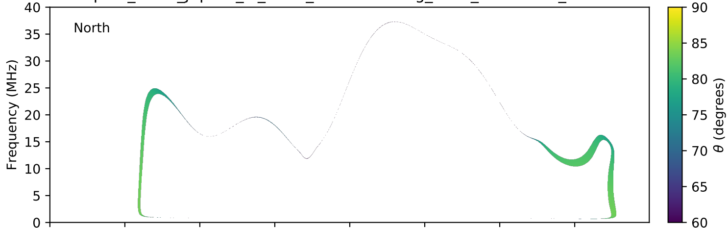
expres_earth_jupiter_io_isaac_lossc-wid1deg_3kev_20100820_v01.cdf
