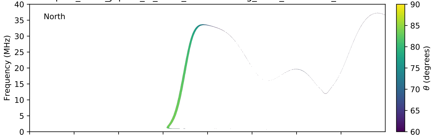
expres_earth_jupiter_io_isaac_lossc-wid1deg_3kev_20100818_v01.cdf
