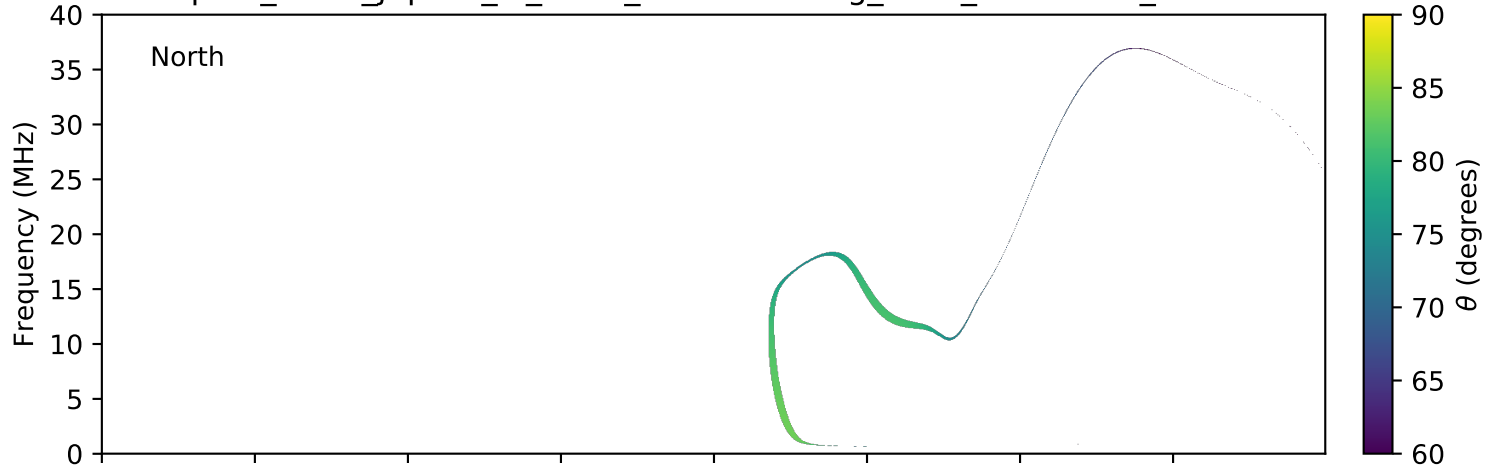
expres_earth_jupiter_io_isaac_lossc-wid1deg_3kev_20100816_v01.cdf
