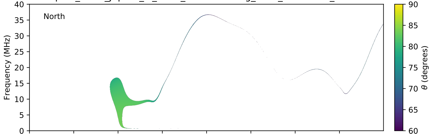
expres_earth_jupiter_io_isaac_lossc-wid1deg_3kev_20100811_v01.cdf
