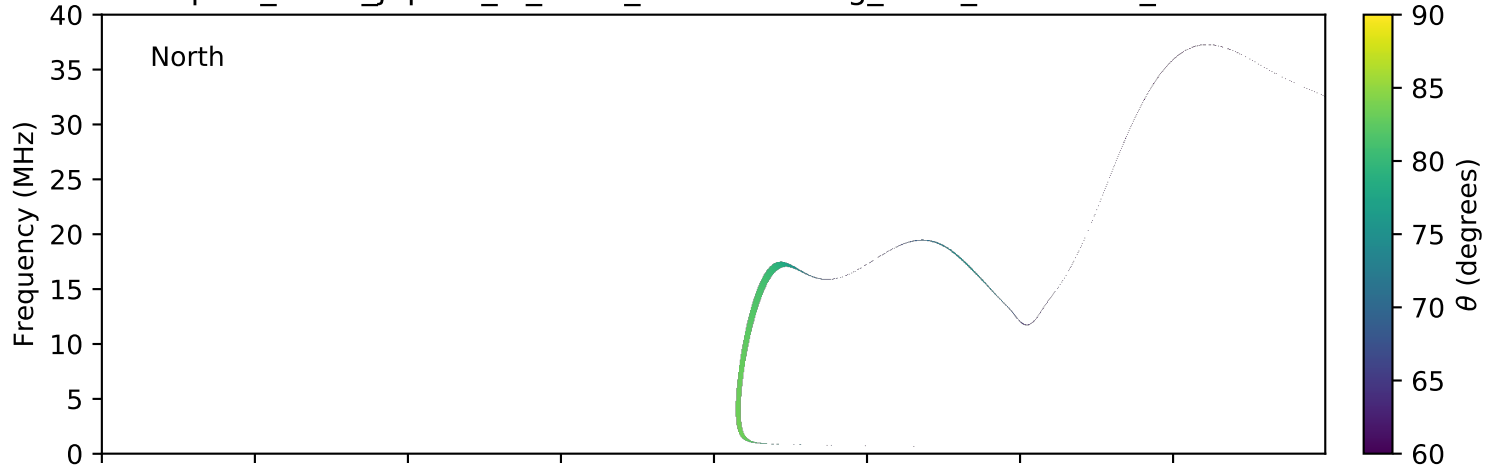
expres_earth_jupiter_io_isaac_lossc-wid1deg_3kev_20100809_v01.cdf
