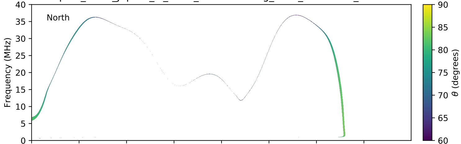
expres_earth_jupiter_io_isaac_lossc-wid1deg_3kev_20100806_v01.cdf
