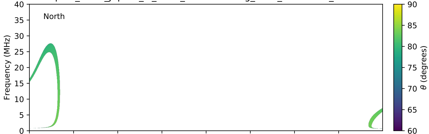
expres_earth_jupiter_io_isaac_lossc-wid1deg_3kev_20100805_v01.cdf
