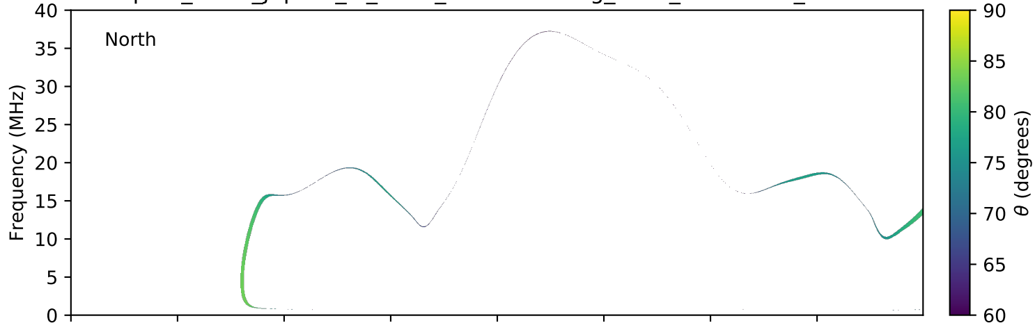
expres_earth_jupiter_io_isaac_lossc-wid1deg_3kev_20100804_v01.cdf
