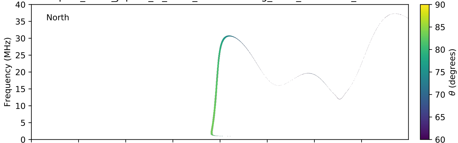
expres_earth_jupiter_io_isaac_lossc-wid1deg_3kev_20100802_v01.cdf
