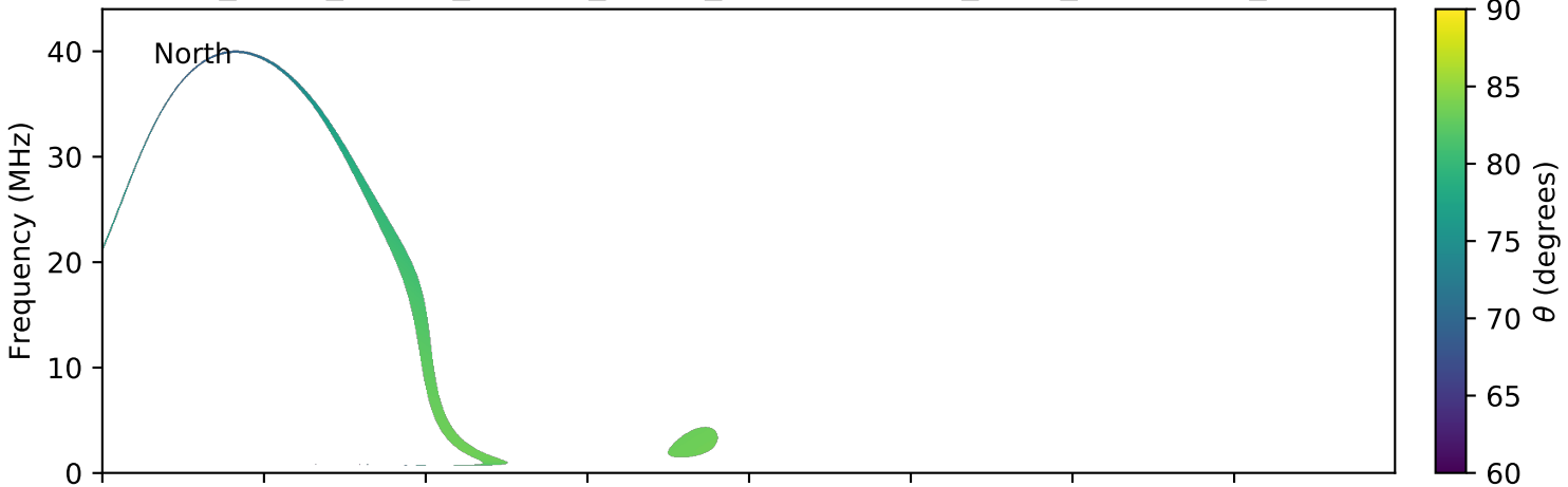
expres_earth_jupiter_europa_jrm09_lossc-wid1deg_3kev_20100811_v01.cdf
