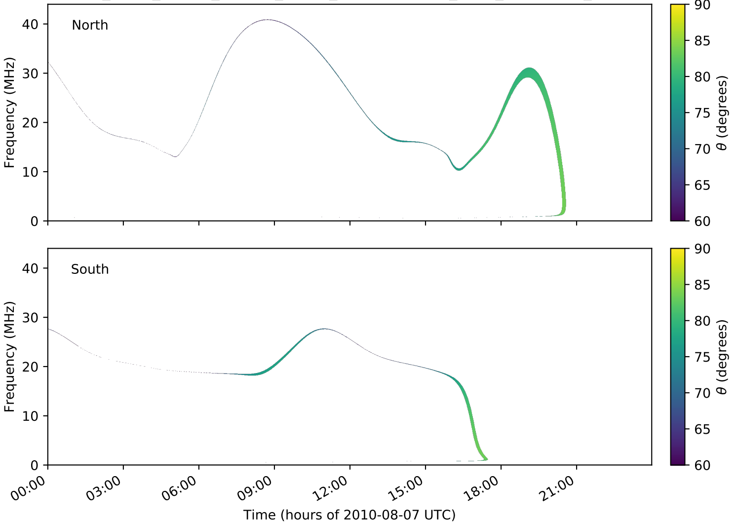
expres_earth_jupiter_europa_jrm09_lossc-wid1deg_3kev_20100807_v01.cdf
