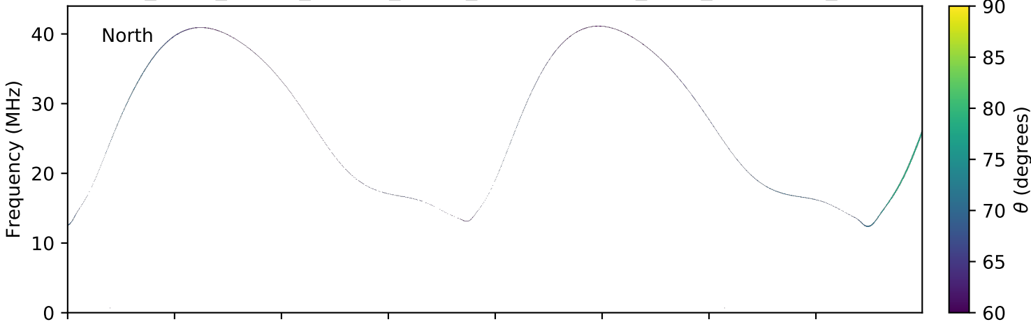
expres_earth_jupiter_europa_jrm09_lossc-wid1deg_3kev_20100803_v01.cdf
