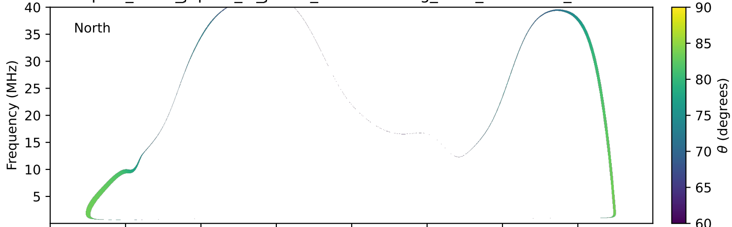
expres_earth_jupiter_io_jrm33_lossc-wid1deg_3kev_20100721_v11.cdf
