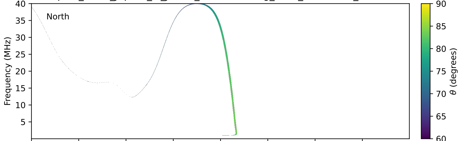
expres_earth_jupiter_io_jrm33_lossc-wid1deg_3kev_20100709_v11.cdf
