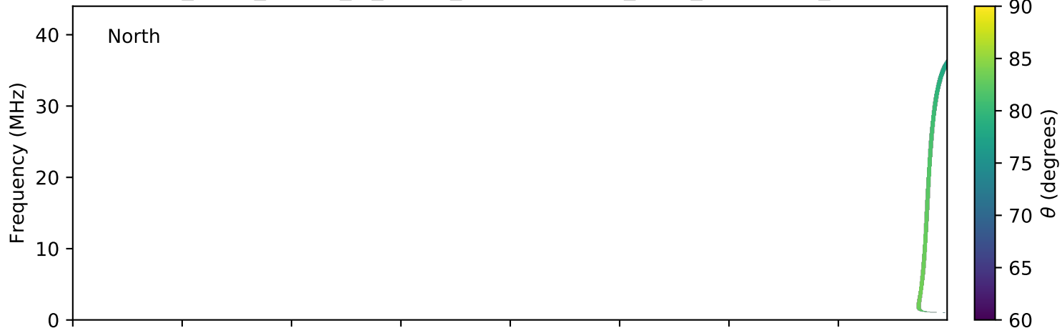
expres_earth_jupiter_io_jrm09_lossc-wid1deg_3kev_20100729_v01.cdf
