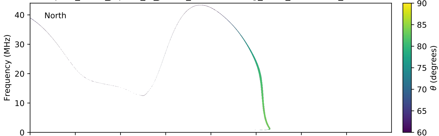
expres_earth_jupiter_io_jrm09_lossc-wid1deg_3kev_20100723_v01.cdf
