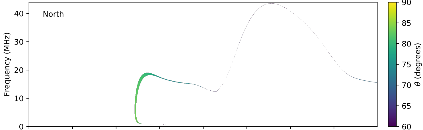
expres_earth_jupiter_io_jrm09_lossc-wid1deg_3kev_20100719_v01.cdf
