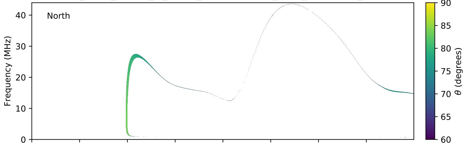
expres_earth_jupiter_io_jrm09_lossc-wid1deg_3kev_20100712_v01.cdf
