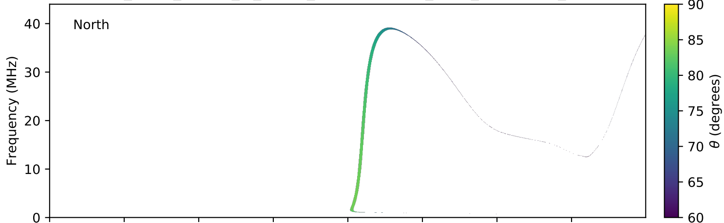
expres_earth_jupiter_io_jrm09_lossc-wid1deg_3kev_20100710_v01.cdf
