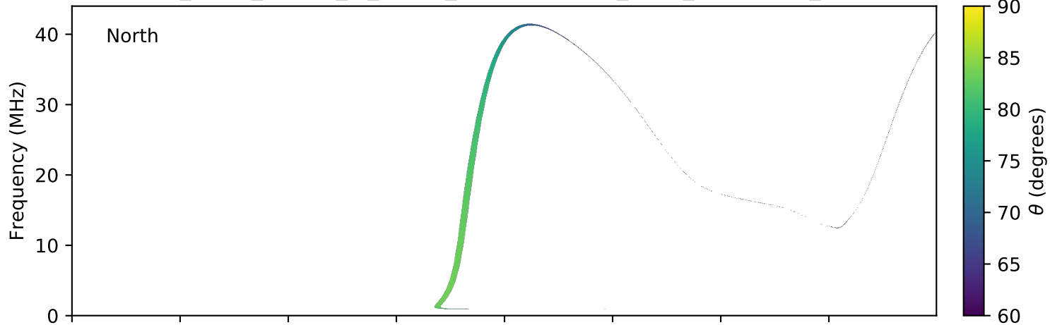
expres_earth_jupiter_io_jrm09_lossc-wid1deg_3kev_20100703_v01.cdf
