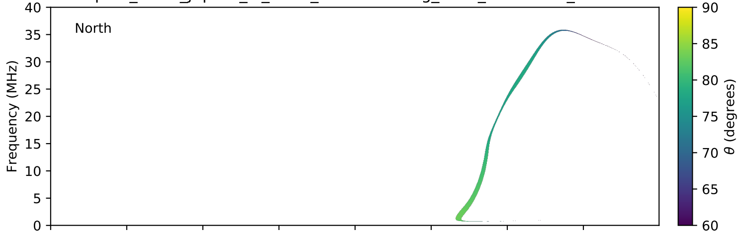
expres_earth_jupiter_io_isaac_lossc-wid1deg_3kev_20100731_v01.cdf
