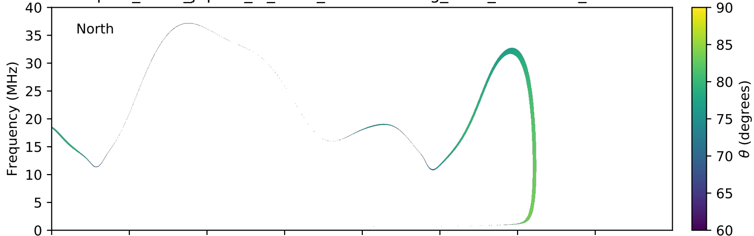
expres_earth_jupiter_io_isaac_lossc-wid1deg_3kev_20100730_v01.cdf
