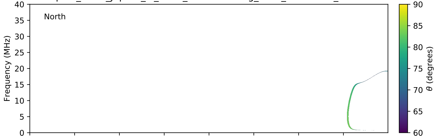
expres_earth_jupiter_io_isaac_lossc-wid1deg_3kev_20100729_v01.cdf
