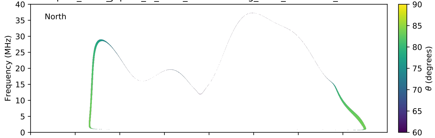
expres_earth_jupiter_io_isaac_lossc-wid1deg_3kev_20100728_v01.cdf
