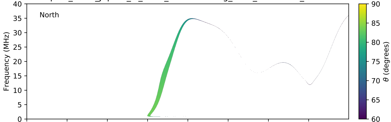
expres_earth_jupiter_io_isaac_lossc-wid1deg_3kev_20100726_v01.cdf
