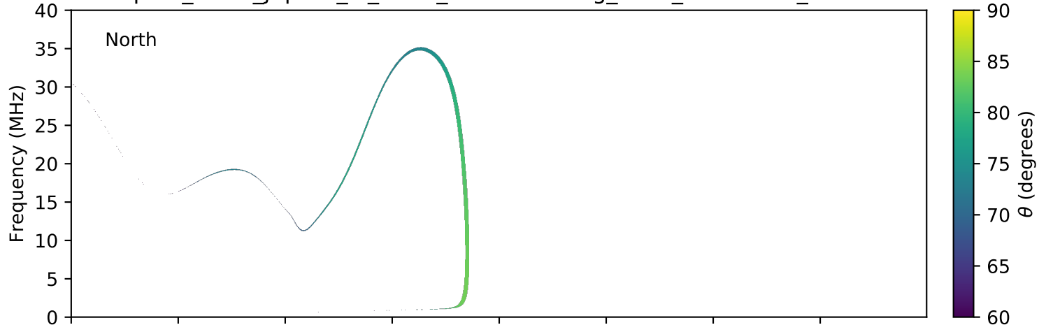
expres_earth_jupiter_io_isaac_lossc-wid1deg_3kev_20100725_v01.cdf
