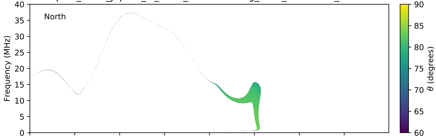
expres_earth_jupiter_io_isaac_lossc-wid1deg_3kev_20100723_v01.cdf
