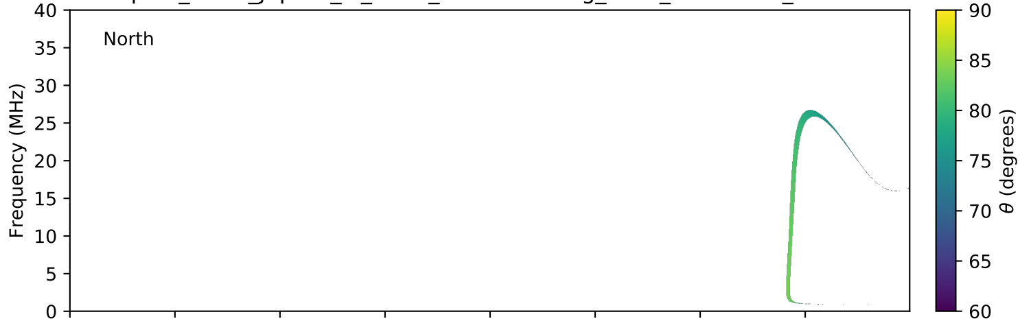
expres_earth_jupiter_io_isaac_lossc-wid1deg_3kev_20100722_v01.cdf
