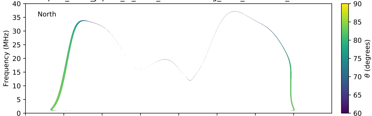
expres_earth_jupiter_io_isaac_lossc-wid1deg_3kev_20100721_v01.cdf
