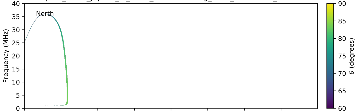
expres_earth_jupiter_io_isaac_lossc-wid1deg_3kev_20100720_v01.cdf
