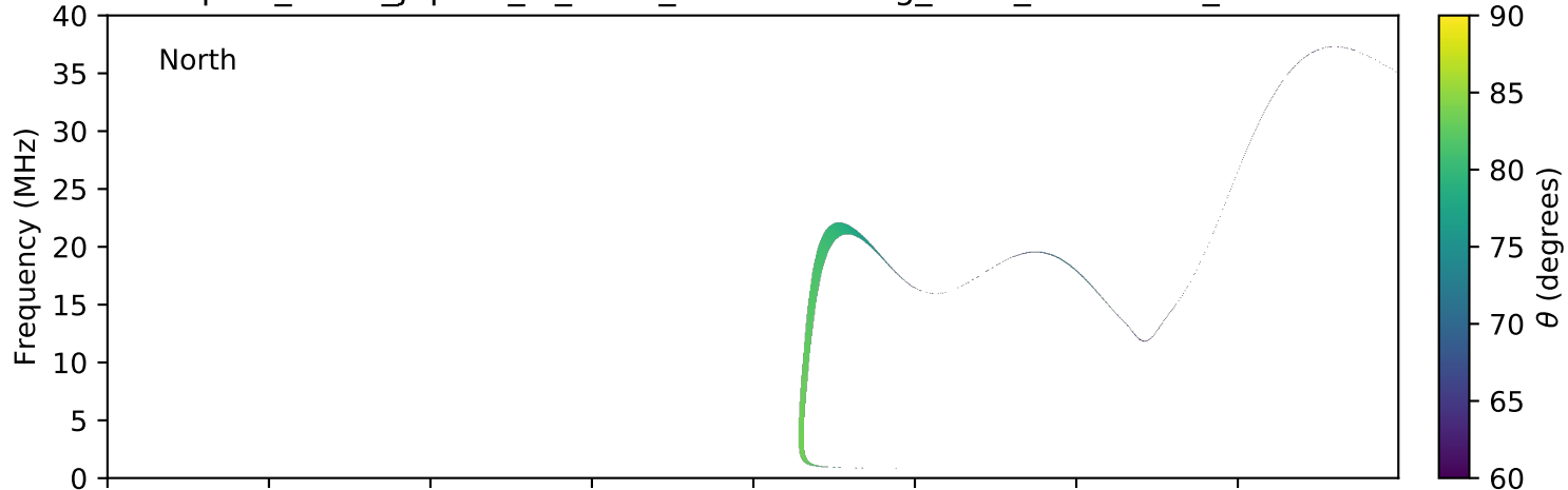
expres_earth_jupiter_io_isaac_lossc-wid1deg_3kev_20100717_v01.cdf
