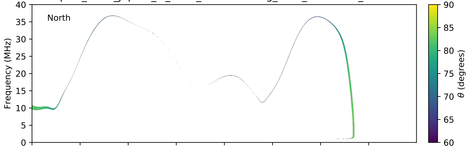
expres_earth_jupiter_io_isaac_lossc-wid1deg_3kev_20100714_v01.cdf
