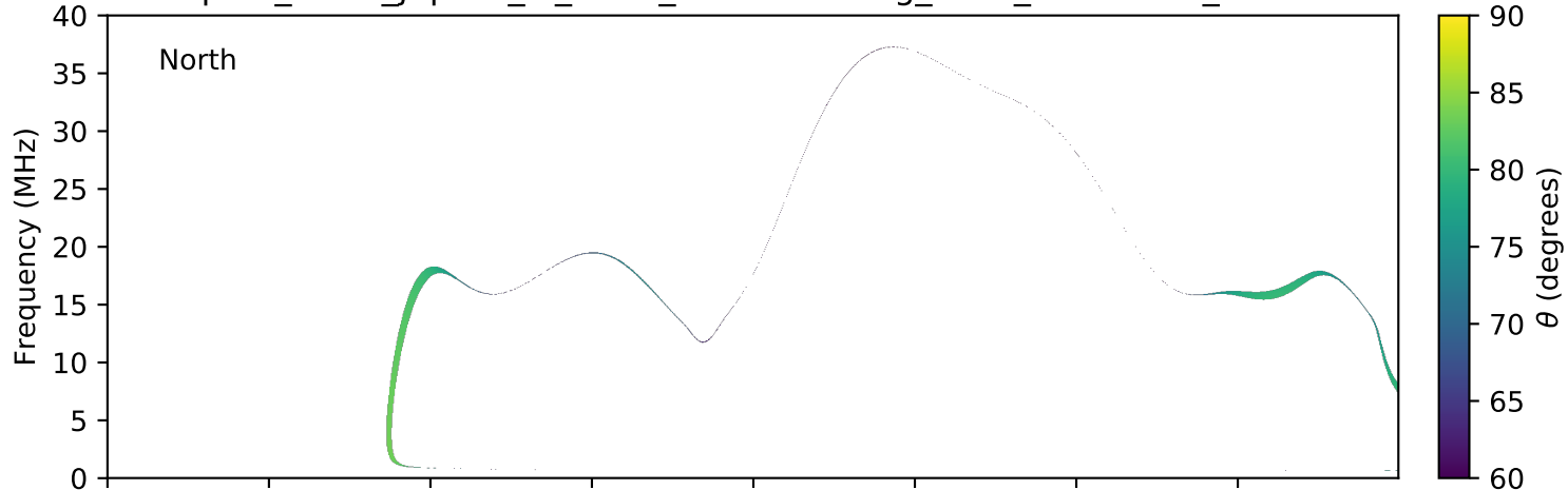
expres_earth_jupiter_io_isaac_lossc-wid1deg_3kev_20100712_v01.cdf
