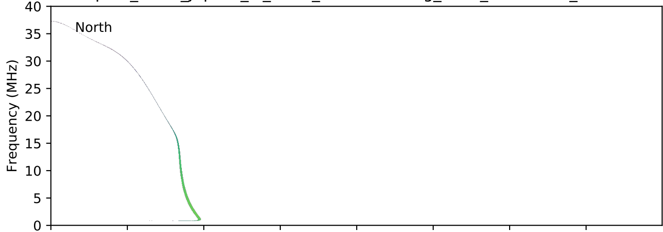
expres_earth_jupiter_io_isaac_lossc-wid1deg_3kev_20100711_v01.cdf
