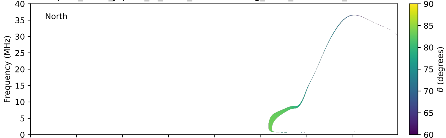
expres_earth_jupiter_io_isaac_lossc-wid1deg_3kev_20100708_v01.cdf
