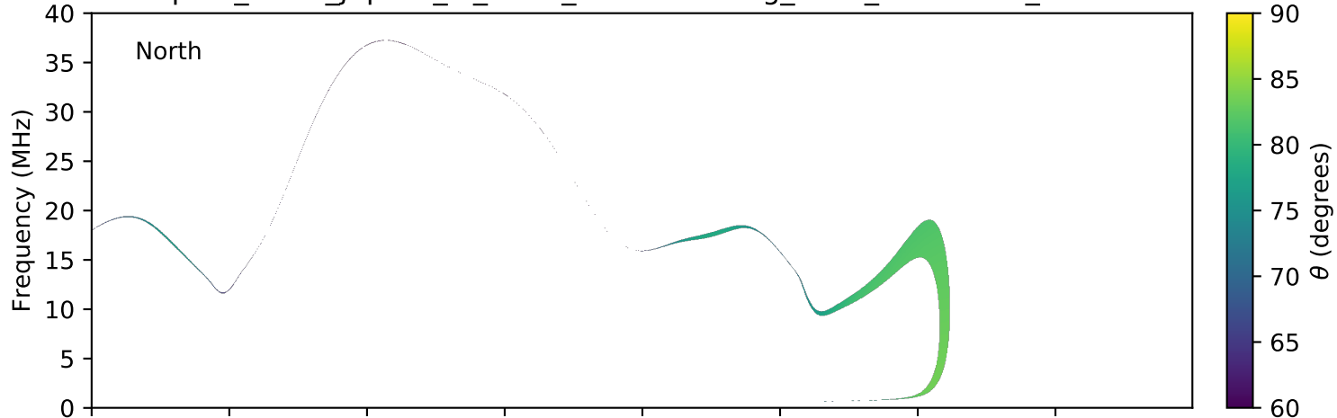
expres_earth_jupiter_io_isaac_lossc-wid1deg_3kev_20100707_v01.cdf
