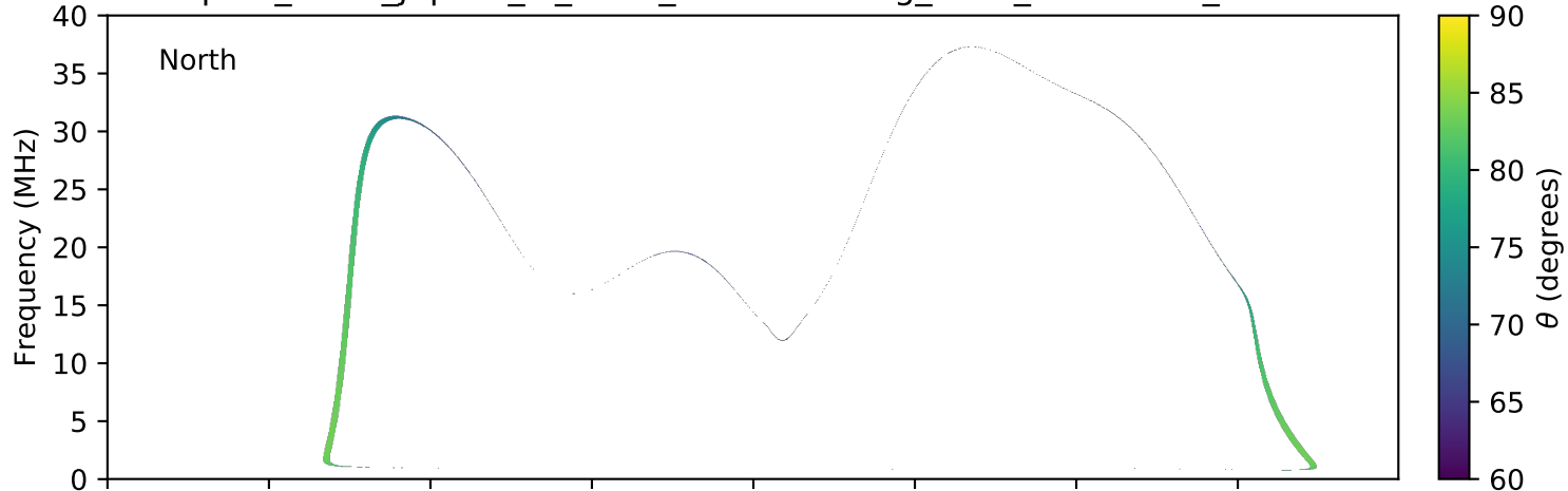
expres_earth_jupiter_io_isaac_lossc-wid1deg_3kev_20100705_v01.cdf
