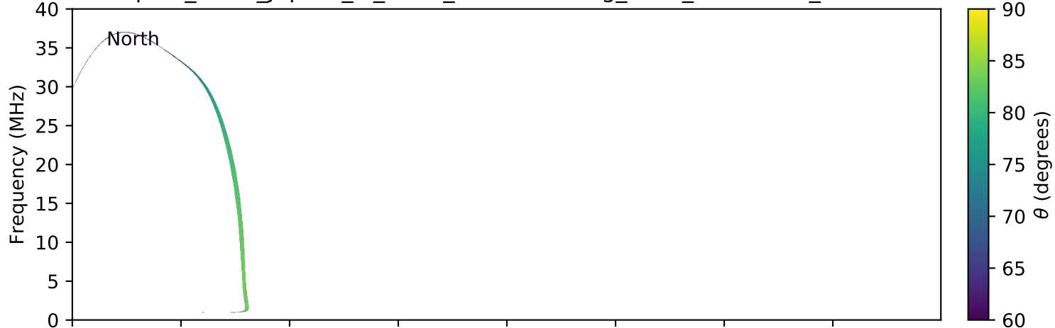
expres_earth_jupiter_io_isaac_lossc-wid1deg_3kev_20100704_v01.cdf
