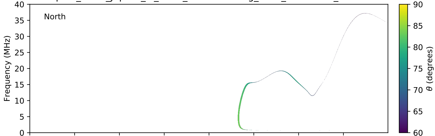
expres_earth_jupiter_io_isaac_lossc-wid1deg_3kev_20100701_v01.cdf
