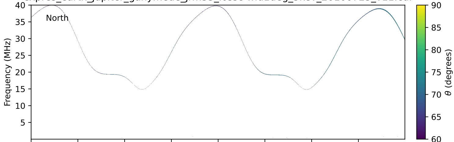
expres_earth_jupiter_ganymede_jrm33_lossc-wid1deg_3kev_20100723_v11.cdf
