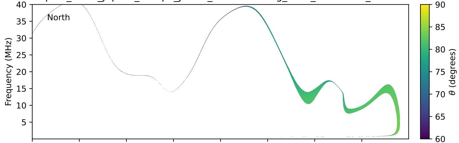
expres_earth_jupiter_europa_jrm33_lossc-wid1deg_3kev_20100706_v11.cdf
