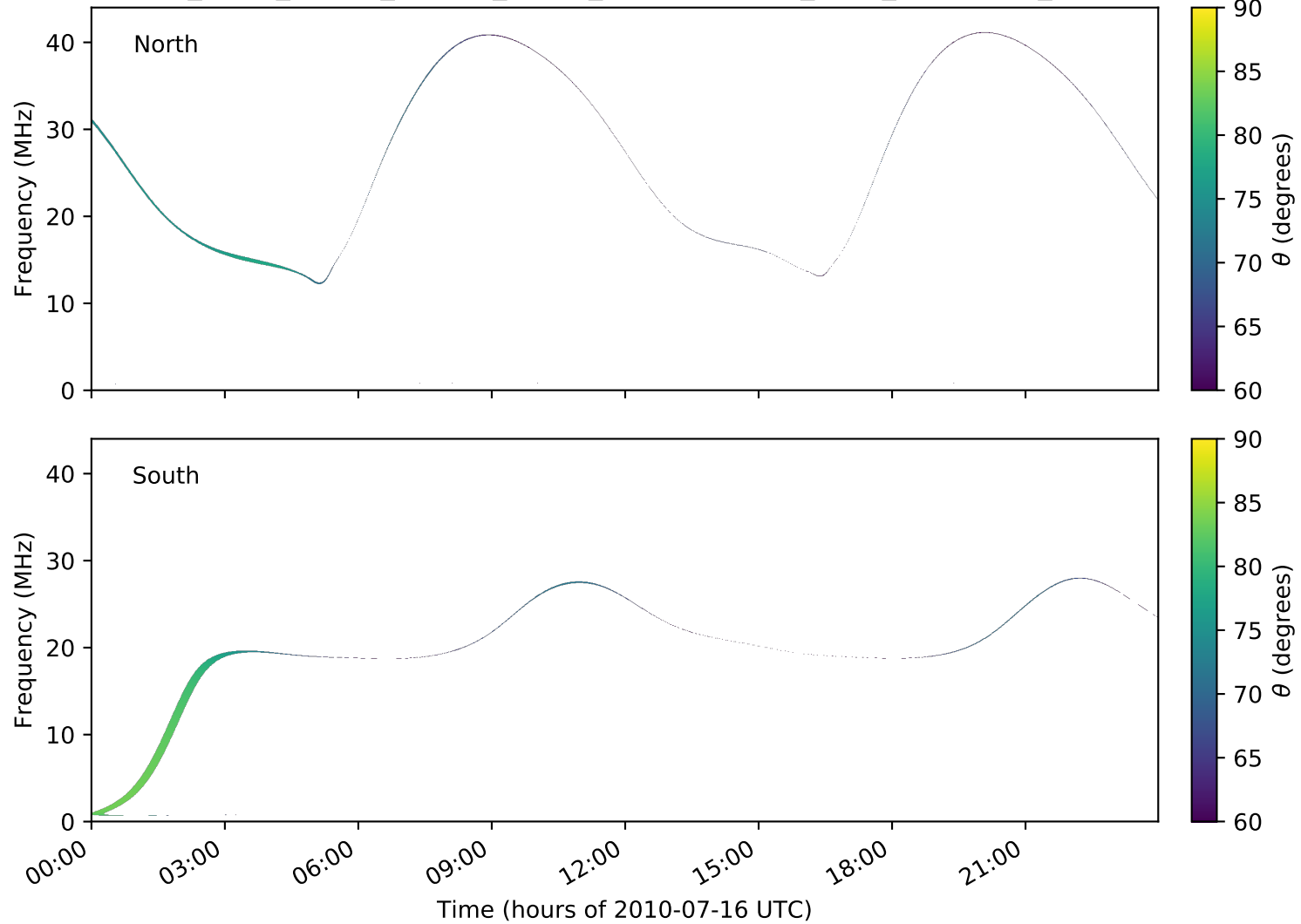
expres_earth_jupiter_europa_jrm09_lossc-wid1deg_3kev_20100716_v01.cdf
