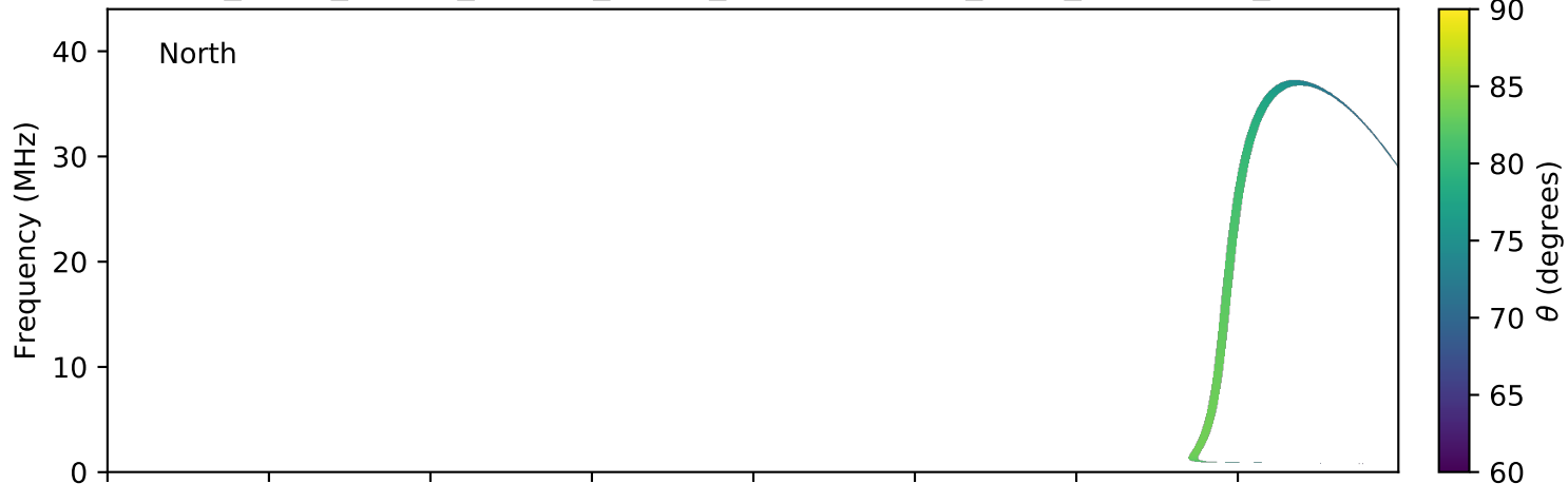
expres_earth_jupiter_europa_jrm09_lossc-wid1deg_3kev_20100708_v01.cdf
