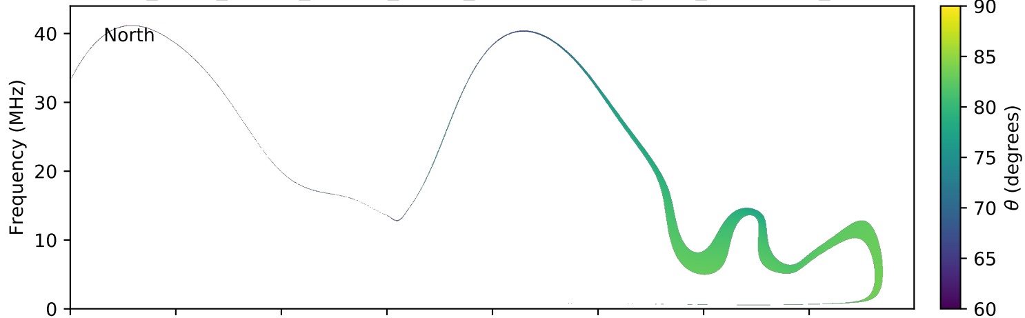
expres_earth_jupiter_europa_jrm09_lossc-wid1deg_3kev_20100706_v01.cdf
