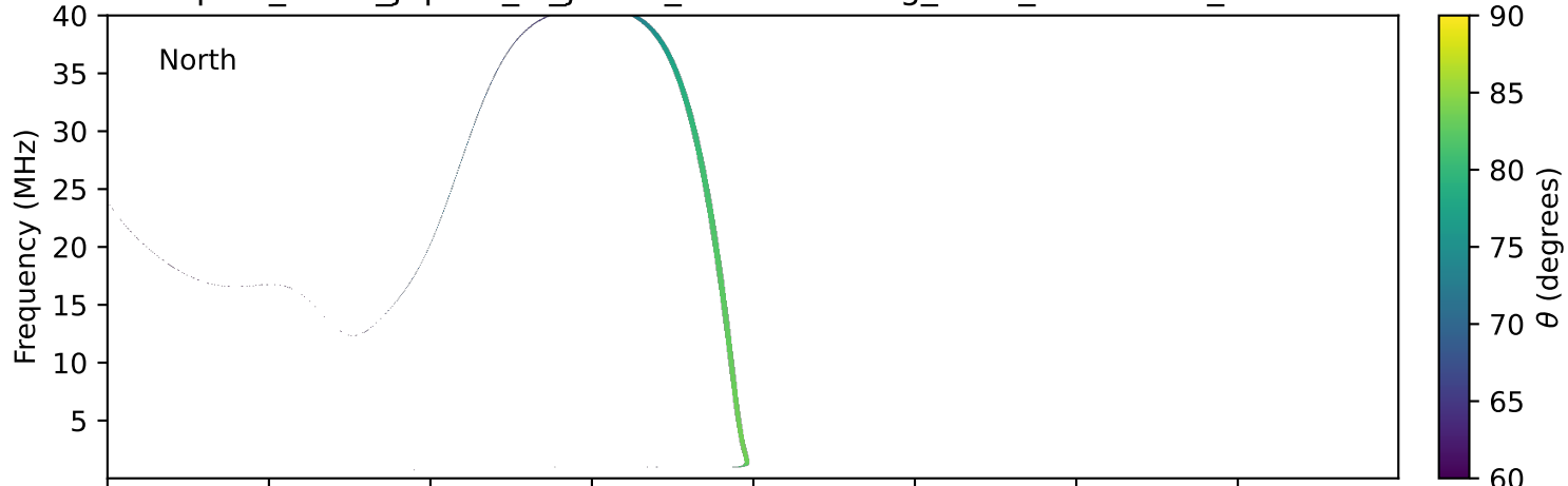
expres_earth_jupiter_io_jrm33_lossc-wid1deg_3kev_20100501_v11.cdf
