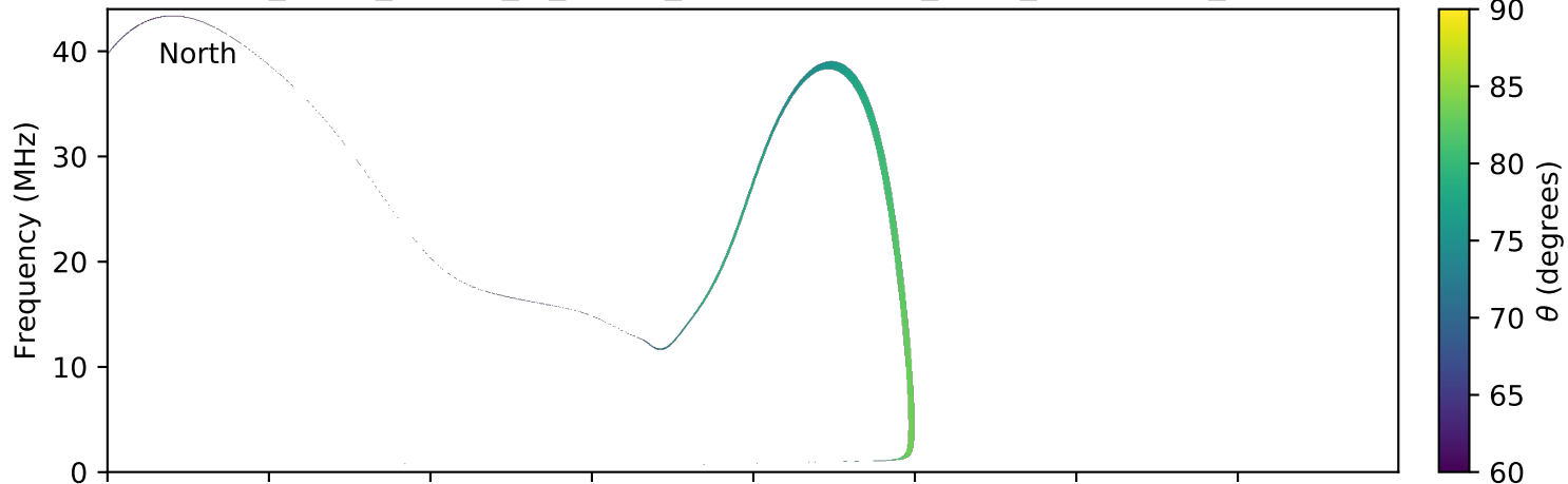
expres_earth_jupiter_io_jrm09_lossc-wid1deg_3kev_20100531_v01.cdf
